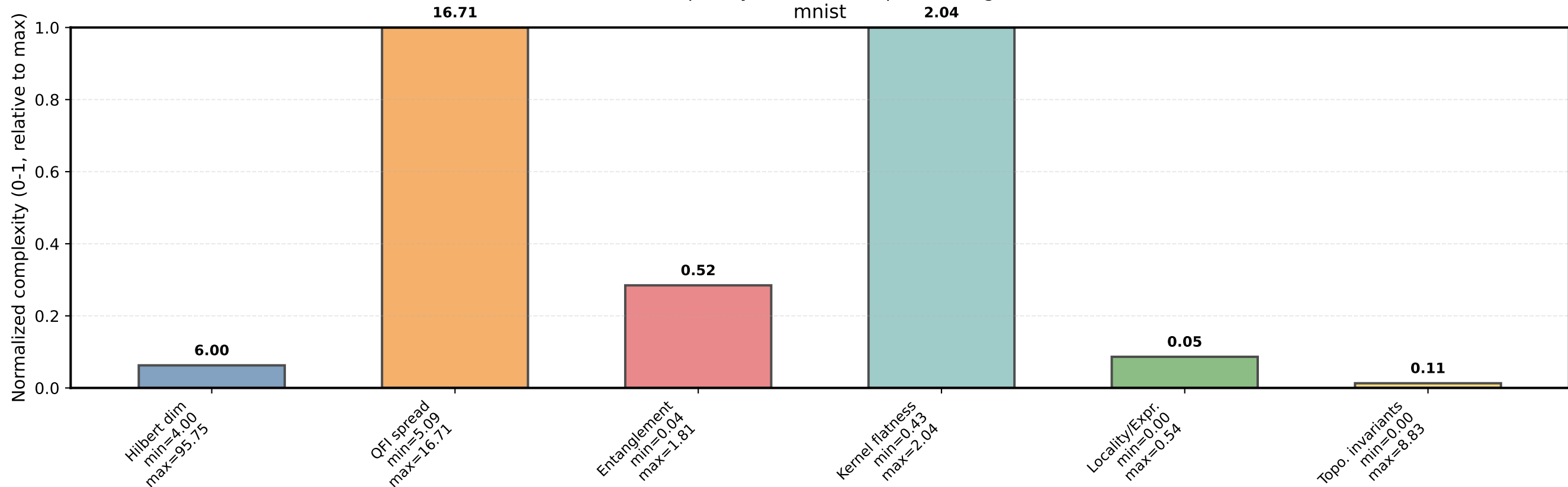
Complexity metrics for nqe encoding
